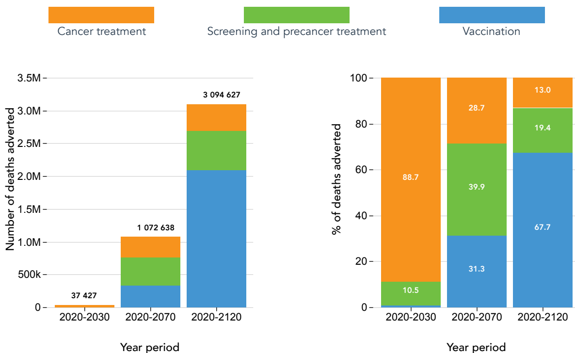
Figure 1: A: Cumulative lives saved if the WHO elimination strategy is implemented. B: Contribution of each elimination pillar to the number of lives saved in Indonesia if the elimination strategy were implemented in 2020.
